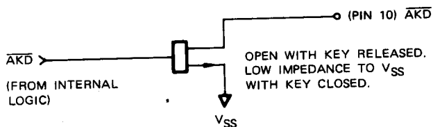
Figure 5. \overline{\text{AKD}} Output Structure
