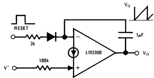
Sawtooth Generator
