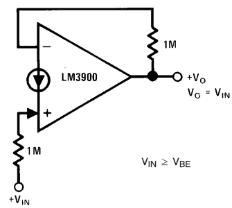
Buffer Amplifier
