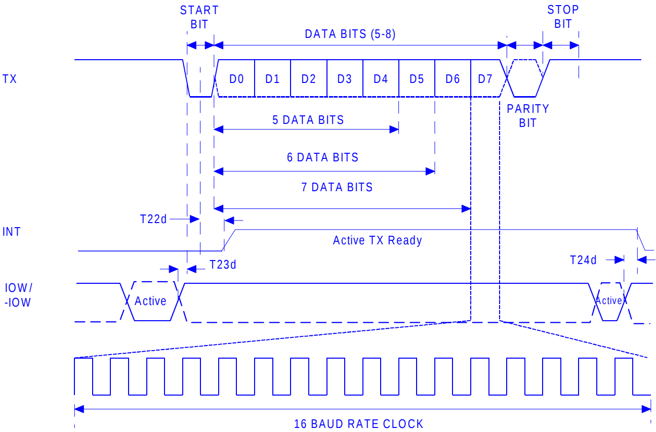
Transmit timing
