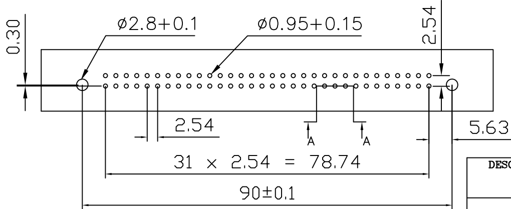
RECOMMENDED PCB HOLE LAYOUT COMPONENT SIDE SCALE 1 : 1
